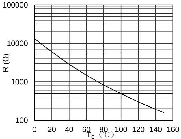
Figure 11. NTC Characteristics
