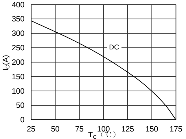
Figure 12. Collector Current vs Case temperature IGBT
