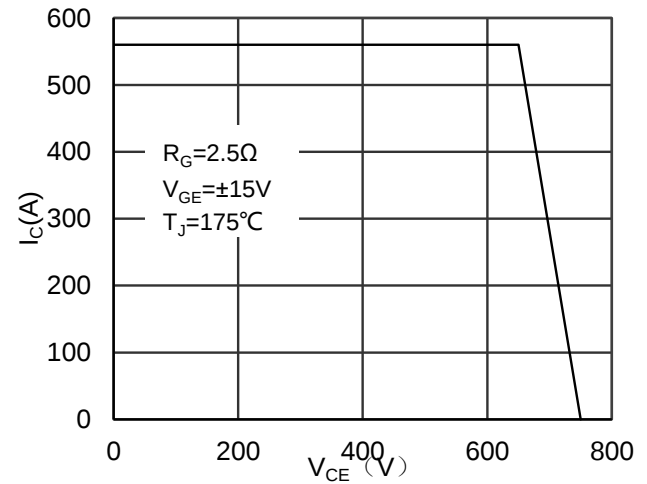
Figure 6. Reverse Bias Safe Operating Area IGBT
