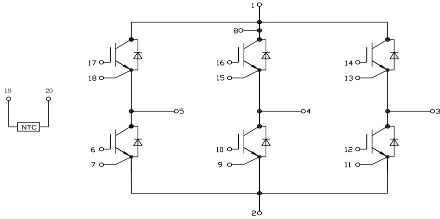
Figure 13. Circuit Diagram
