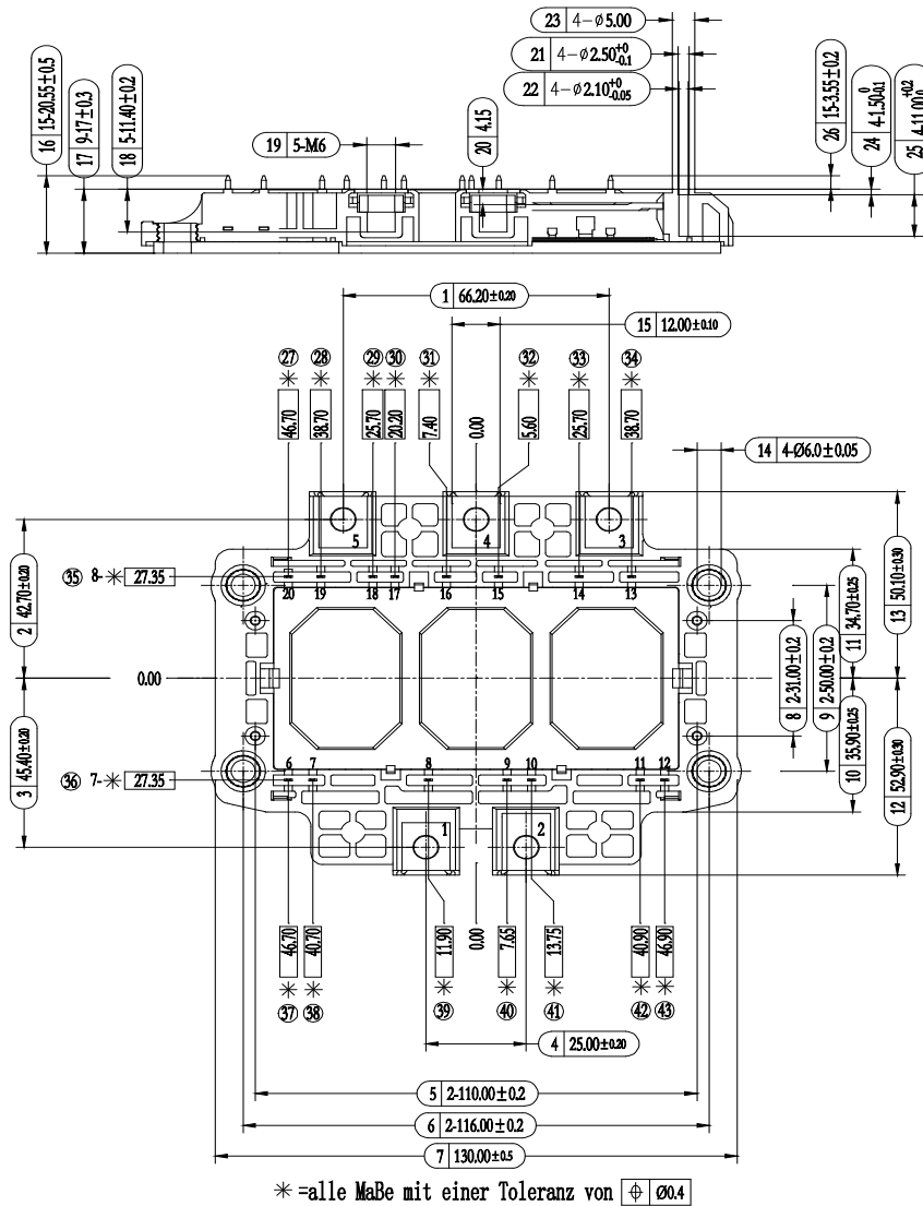
Dimensions in (mm) Figure 14. Package Outline
