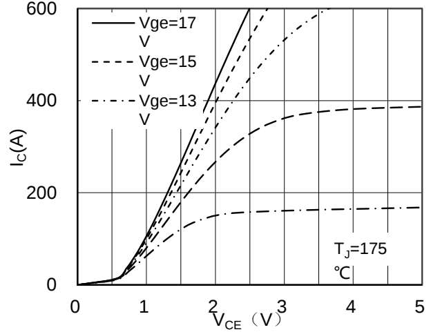
Figure 2. Typical Output Characteristics IGBT
