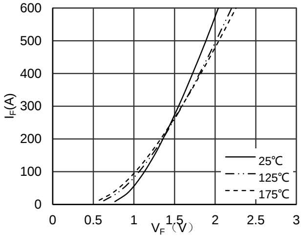
Figure 7. Diode Forward Characteristics Diode
