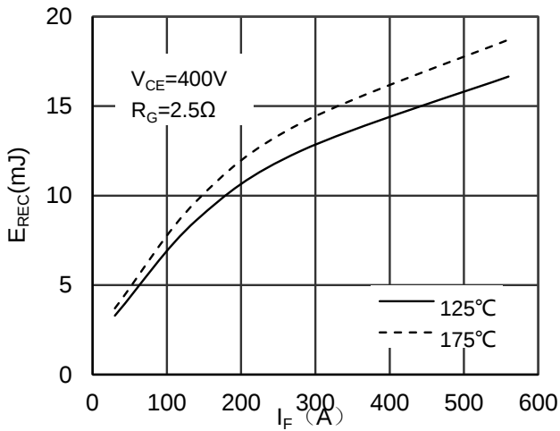
Figure 9. Switching Energy vs Forward Current Diode
