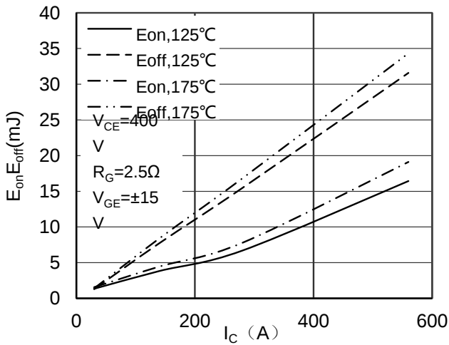
Figure 5. Switching Energy vs Collector Current IGBT
